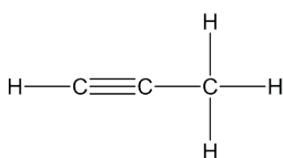
propin
