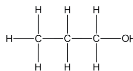
propan-1-ol
